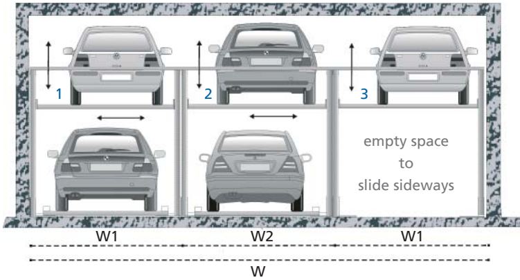
Width dimensions, fig. 3 segments for 5 parking spaces
